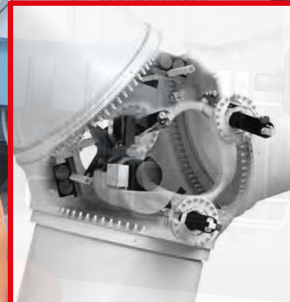
Pitch Cylinders
